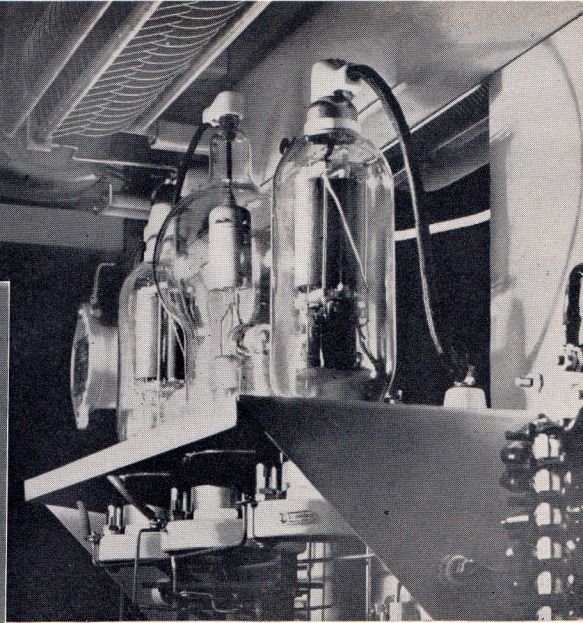
The final amplifier and modulators are in the illustration above. A single type 450TH or 250TH may be used for the final amplifier without making any mechanical or electrical changes. The modulators are 810 tubes.
